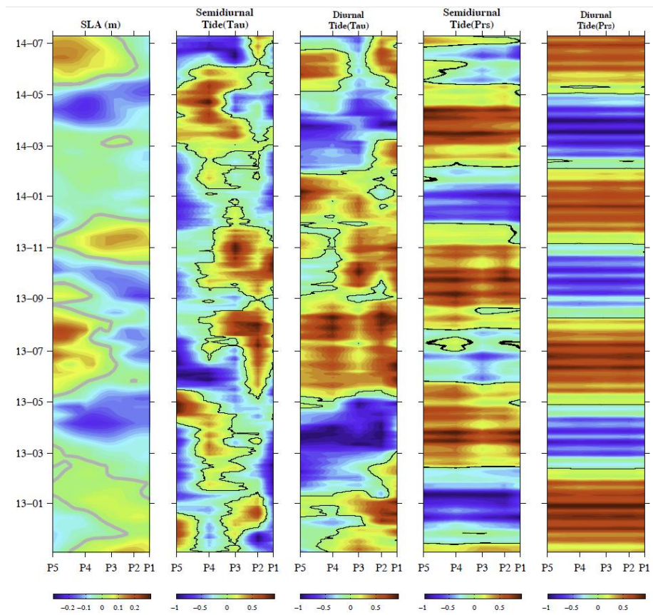
Figure 3. The Hovmöller diagram of the normalized (a) sea level anomaly (b)
