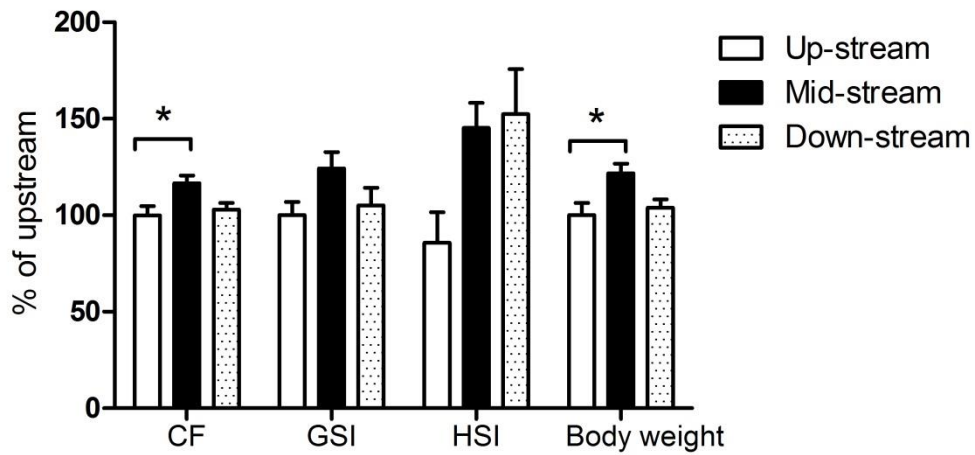
Fig. 2. Condition factor (CF), gonado-somatic index (GSI), hepatosomatic index (HSI) and body weight (BW) expressed as a percentage of values in sharpbelly collected from the mid- and down-streams relative to those in the up-stream. Data represent mean \pm standard deviation (n = 15).
