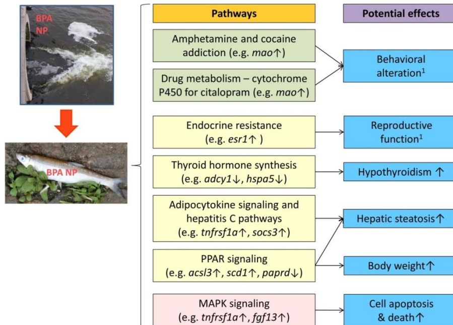
Fig. 4. Schematic diagram of the pathways activated in the female sharpbelly living in the mid-stream. acs3 : Long-chain-fatty-acid--CoA ligase 3; adcy1 : adenylate cyclase 1; esr1 : estrogen receptor 1; fgf13 : Fibroblast growth factor 13; hspa5 : heat shock protein family A (Hsp70) member 5; mao : monoamine oxidase; ppard : Peroxisome proliferator-activated receptor delta; scd1 : stearoyl-CoA desaturase; socs3 : suppressor of cytokine signaling 3; tnfrsf1a : tumor necrosis factor receptor superfamily member 1A. 1. Effects of WWTP effluent on the behavioral alteration and reproductive function were unclear.
