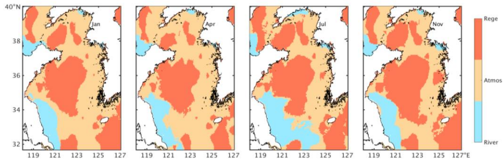
Fig. 10 Distribution of dominant external DIN input
